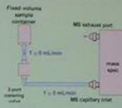
Figure 2. Schematic diagram of the system configured for sampling in static mode.
