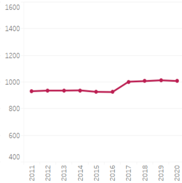
Average SAT
