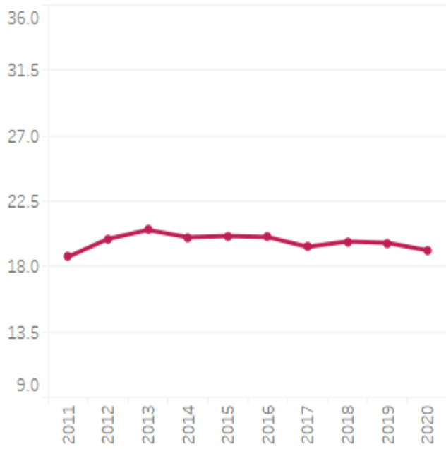
Average ACT
